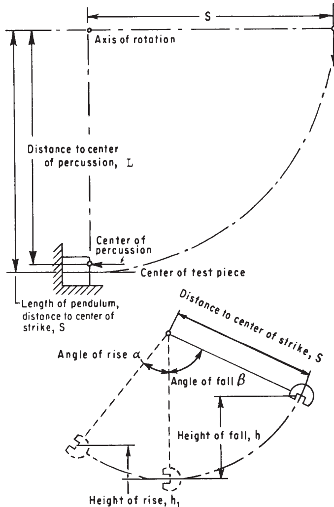
FIG. A2.1 Dimensions for Calculations
