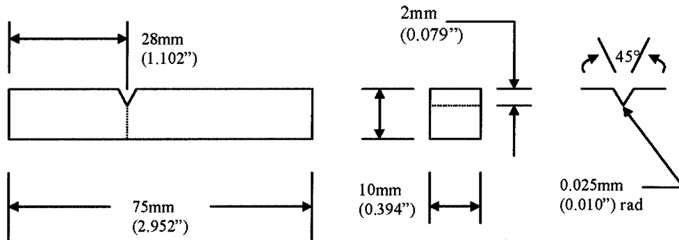
FIG. 1 Charpy (Simple-Beam) Impact Test Specimens, Types A, B, and C
