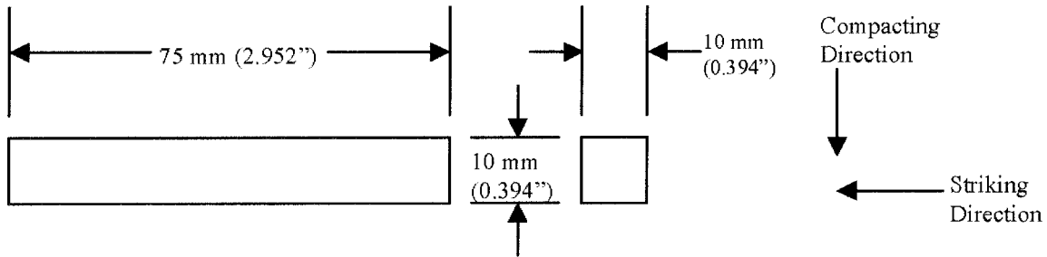
FIG. 4 Charpy (Simple Beam) Impact Test Specimens for Metal Powder Structural Parts
