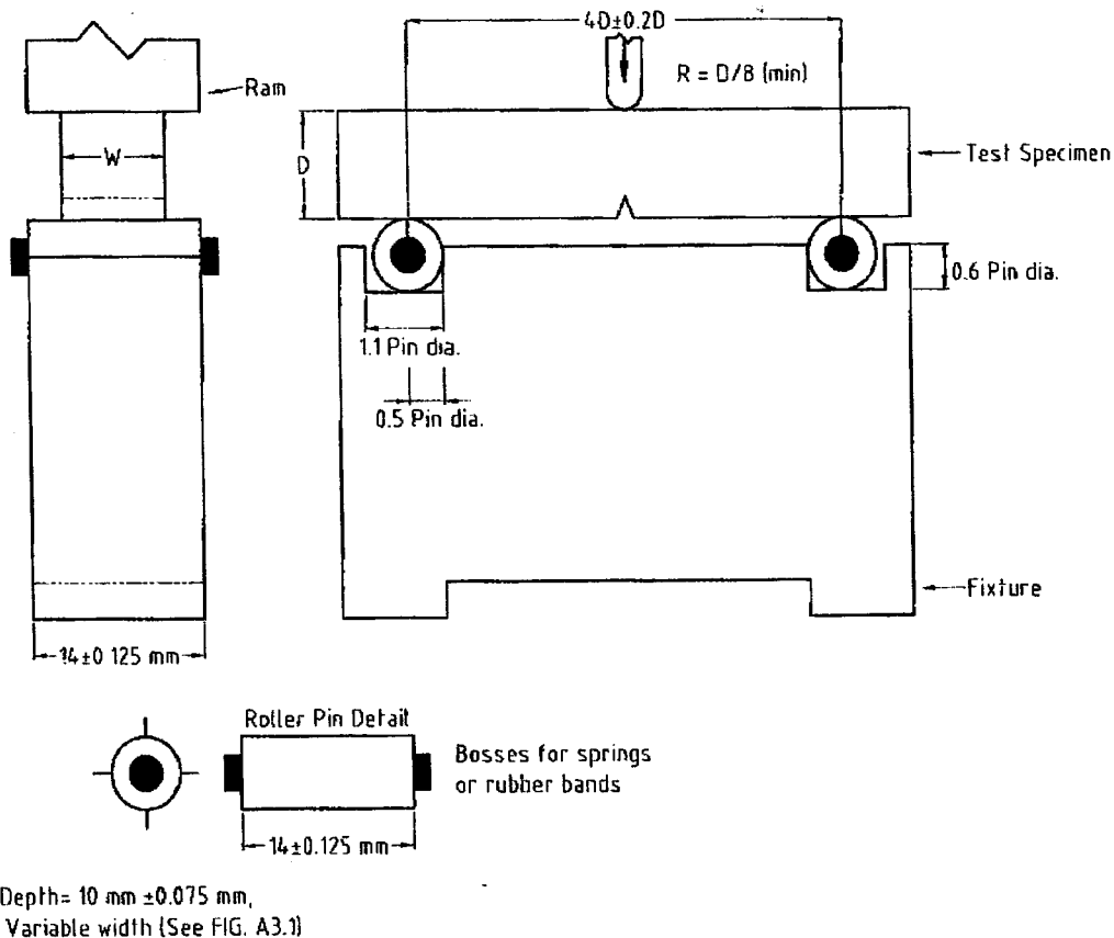
FIG. A4.1 Fatigue Precracking-Fixture Design
