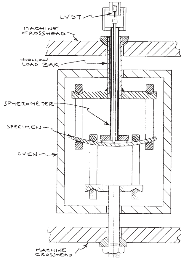
FIG. 7 Specimen and Spherometer in Four-Point to Flexuradingl Stress Fixture
