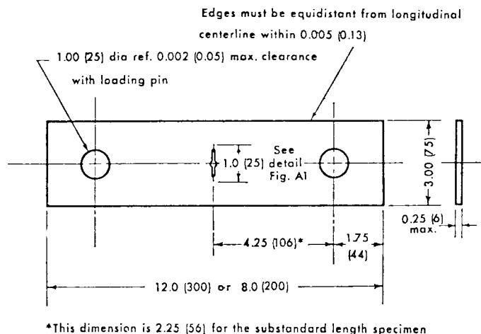
FIG. 4 Fatigue Center-Crack Specimen M(T)
