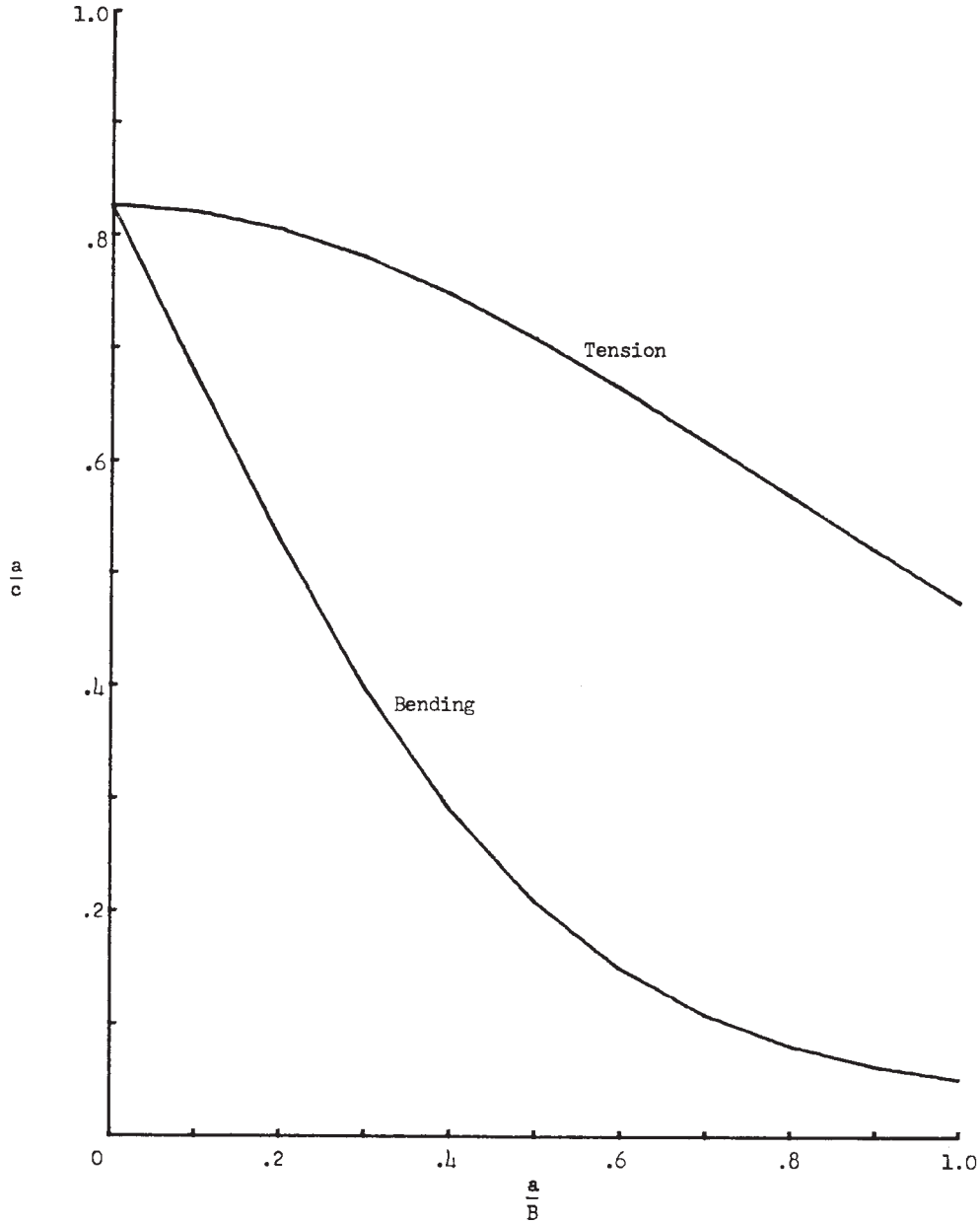
FIG. A2.1 Values of a/c and a/B for Which K is Equal at the Surface and at the Deepest Point on the Crack Periphery
