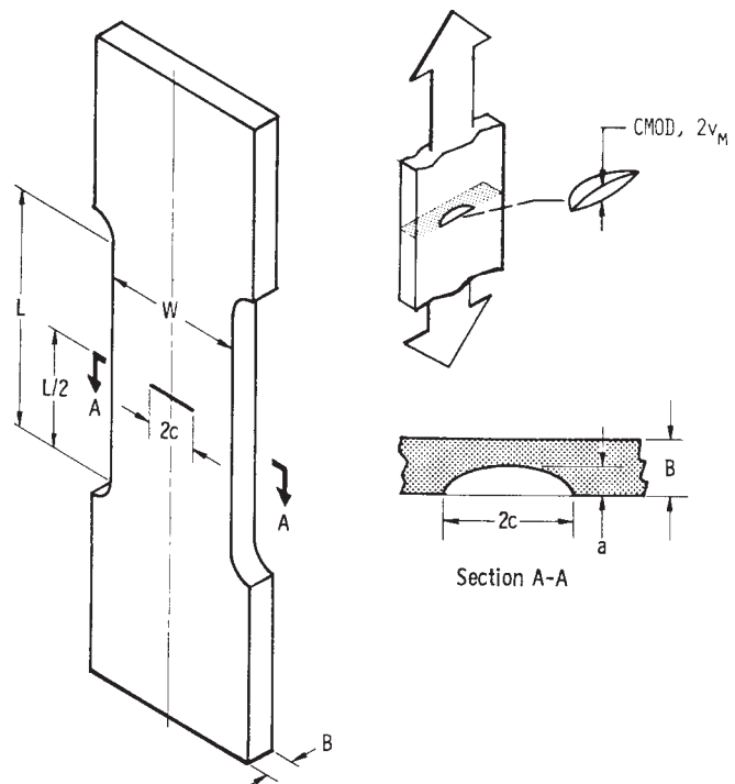
FIG. 1 Typical Surface-Crack Specimen (Grip Details Omitted) and Nomenclature
