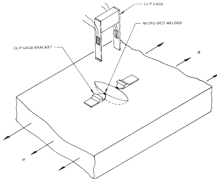
FIG. X2.1 Typical Experimental Setup for CMOD Measurement
