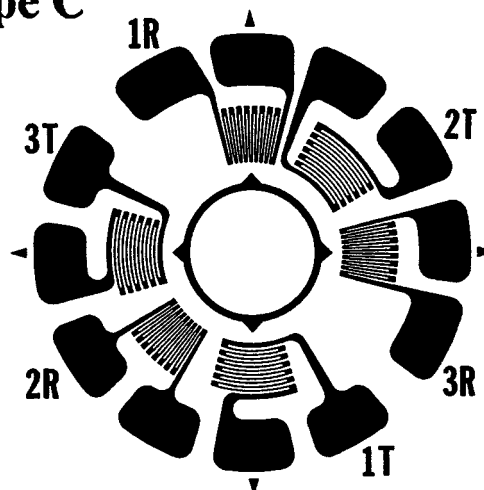
FIG. 3 Hole-Drilling Rosettes
