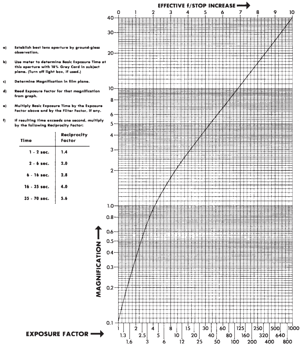
FIG. X2.1 Photomacrography Exposure Computer
