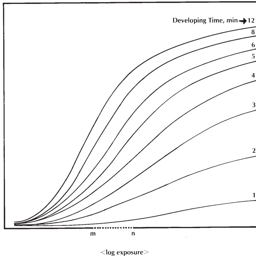
FIG. 2 Optical Density Versus Logarithm of Exposure for Photographic Materials
