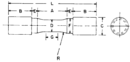
Dimensions, mm
