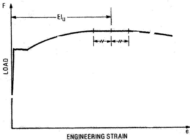
FIG. 27 Load-Strain Diagram for Determination of Uniform Elongation of Steel Sheet Materials Exhibiting a Flat Plateau at Maximum Load
