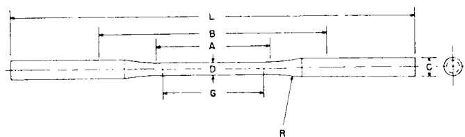
Dimensions, mm
