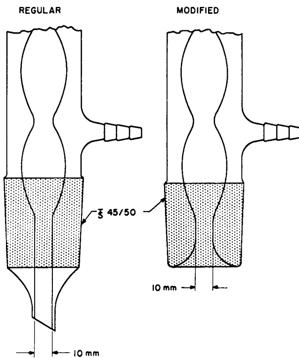
FIG. X1.4 Modification of Allihn Condenser to Prevent Loss of Vapor
