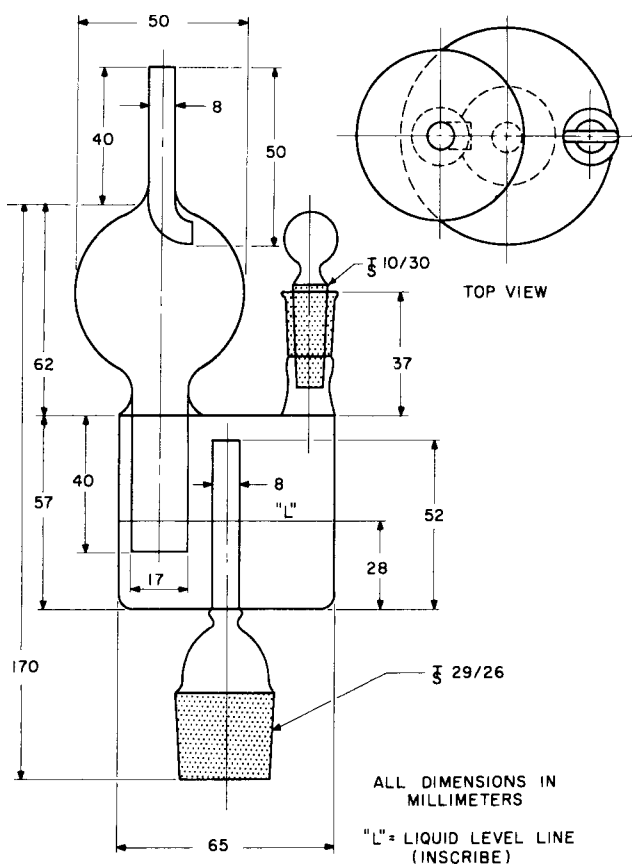
FIG. X1.3 Trap for Top of Condenser to Prevent Loss of Vapor
