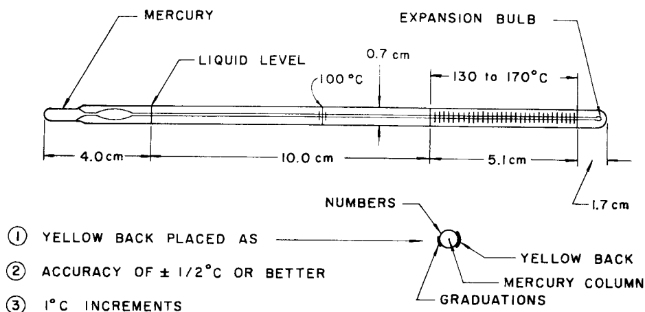
FIG. X1.5 Design of Thermometer for Use in Flask of Fig. X1.2
