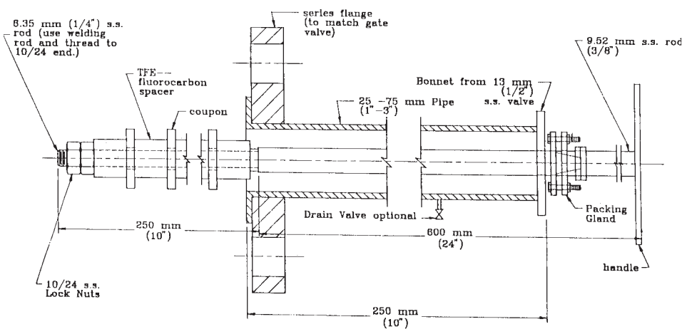
FIG. 4 Retractable "Slip-In" Cou Specimen Holder
