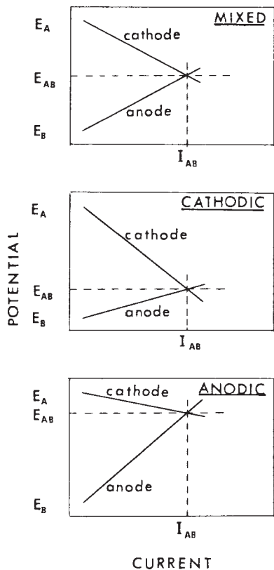
FIG. X1.3 Effects of Polarization on Metal Potential
