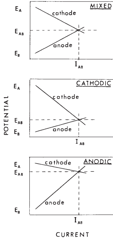
FIG. X1.3 Effects of Polarization on Metal Potential
