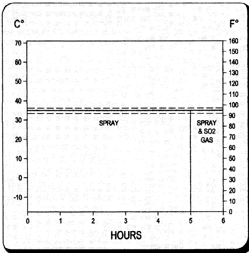
NOTE 1—Dashed chart lines indicate temperature tolerance limits. NOTE 2—© 2000 Singleton Corporation. Used by ASTM with perpetual permission of the Singleton Corporation. FIG. X4.1 Cyclic Salt/SO 2 Spray (Fog) Testing (Example A4.4.4.1)
