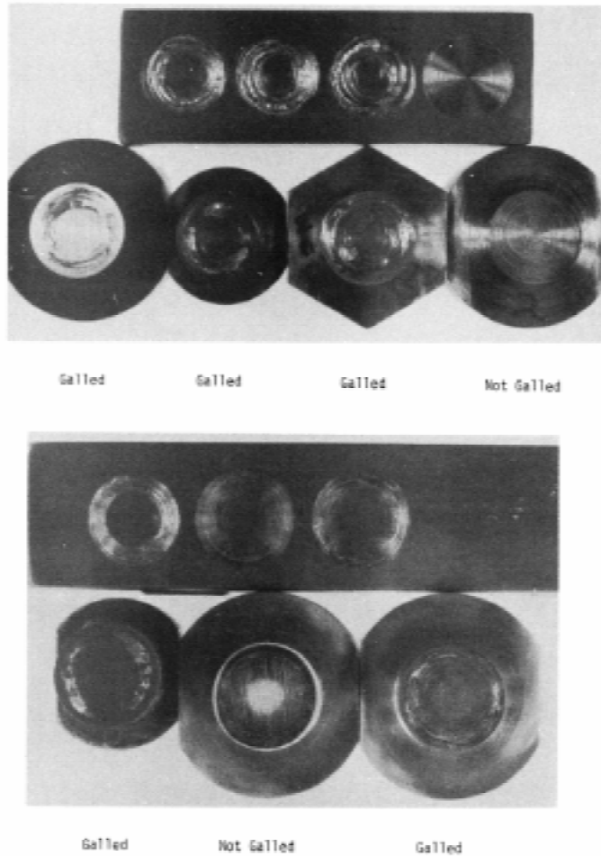
FIG. 4 Test Specimens
