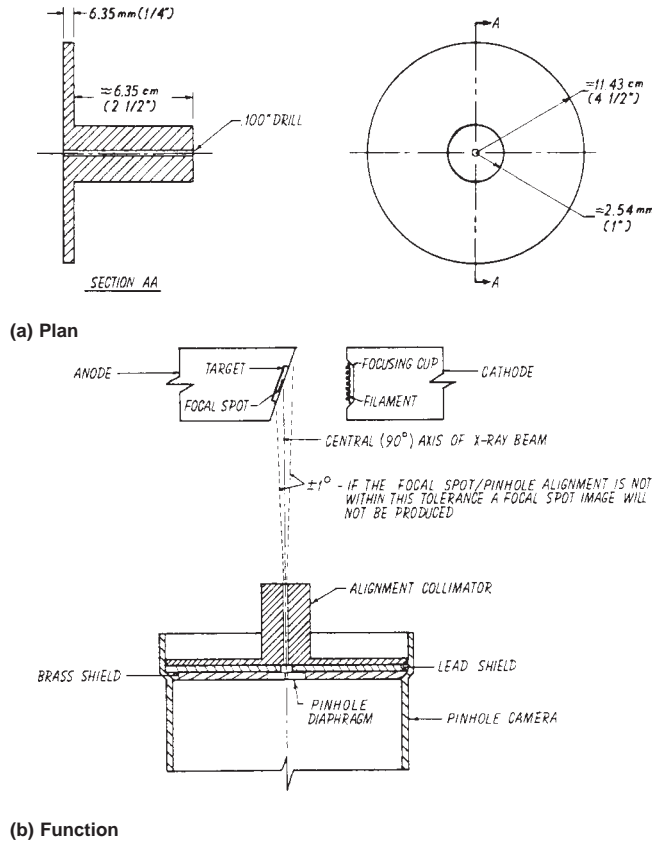
FIG. 7 Alignment Collimator
