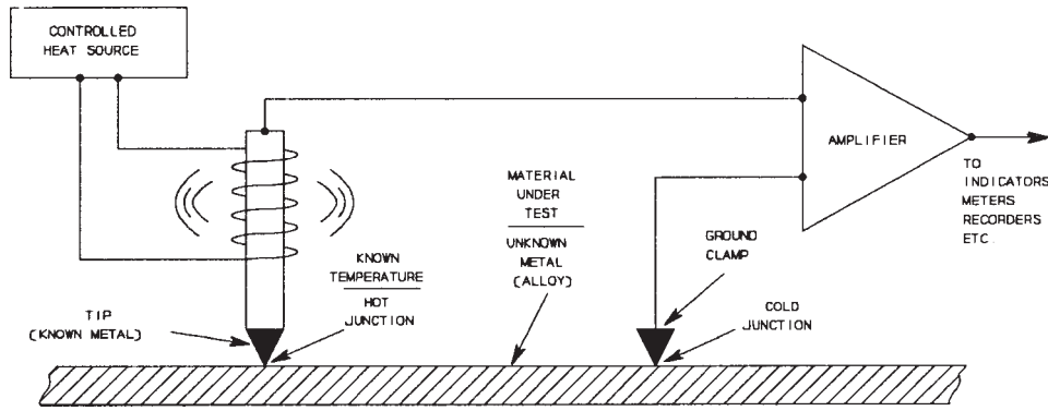
FIG. 3 Typical Circuit used in Thermoelectric Sorting Instruments
