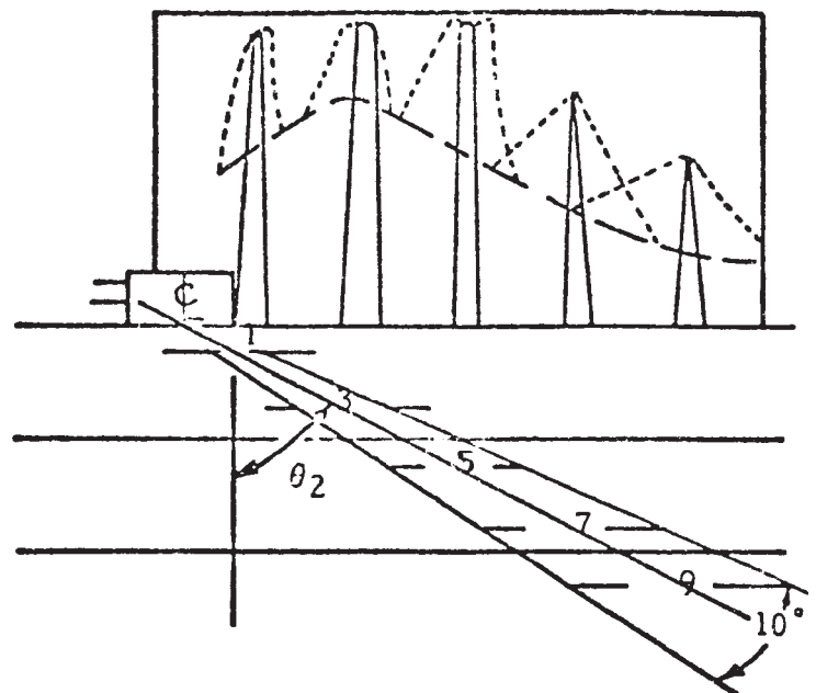
FIG. A2.9 Beam Spread
