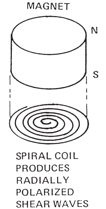
FIG. 4 Diagram of Spiral Coil EMAT
