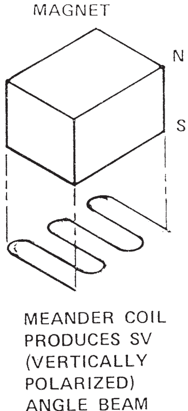
FIG. 5 Diagram of Meander Coil EMAT
