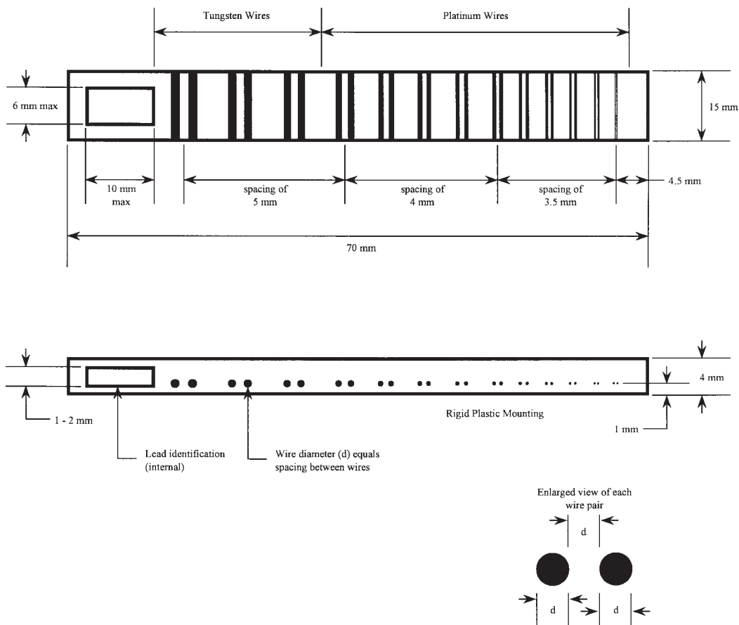
FIG. 1 Total Image Unsharpness Gage (see EN-462-5)
