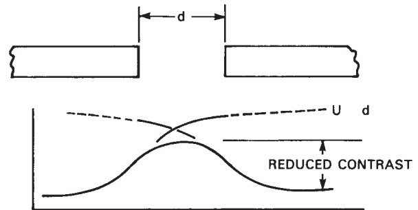
FIG. 3 Effect of Geometric Unsharpness on Image Contrast
