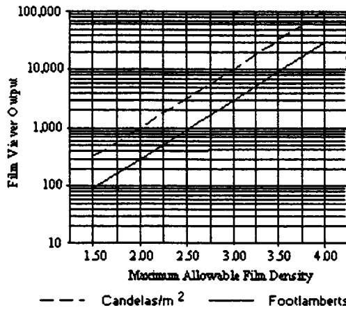
FIG. 1 Maximum Film Density Allowable with Film Viewer
