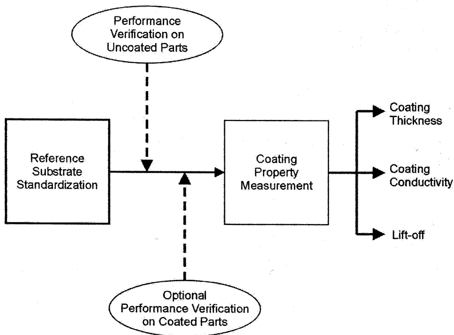
FIG. X2.3 Coating Characterization Procedure—Reference Substrate Standardization
