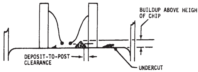
FIG. 5 Transistor—Mounting Paste Buildup or Expulsion or Both
