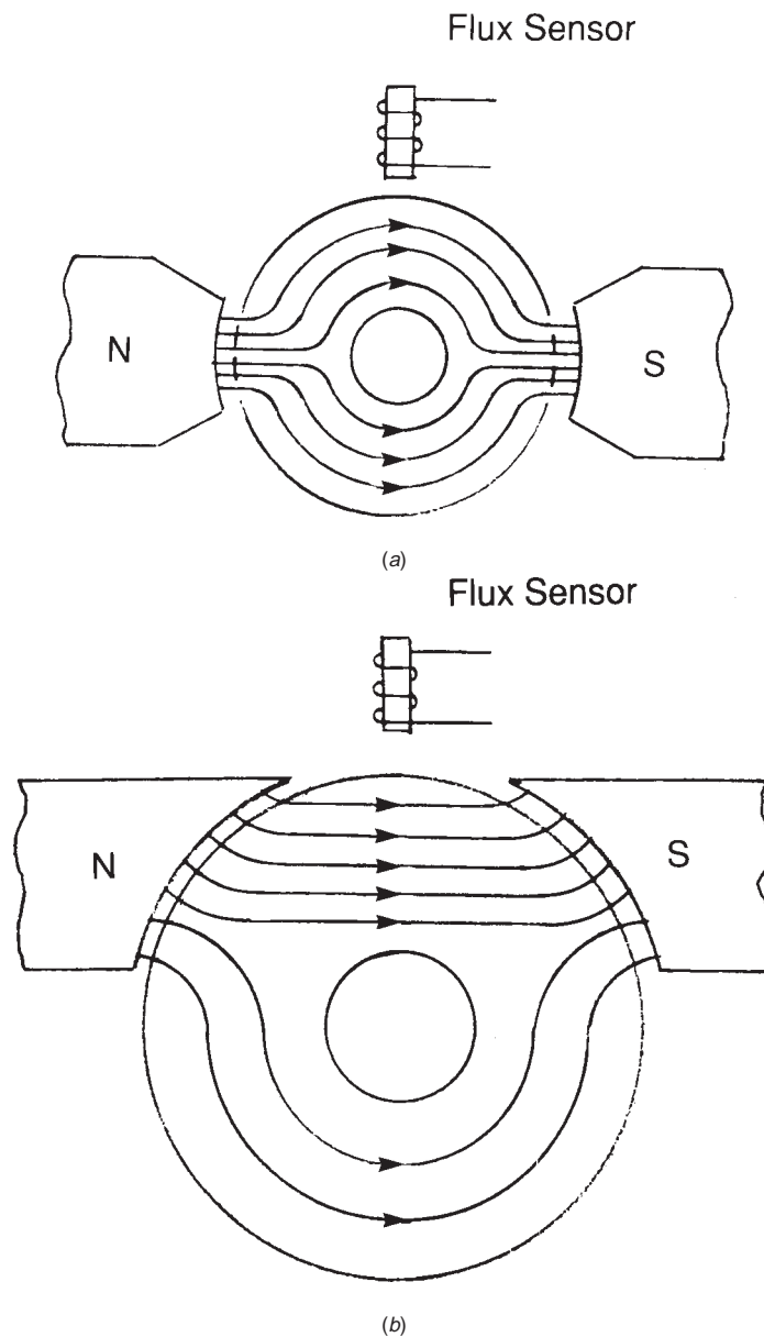
FIG. 1 Transverse Magnetization
