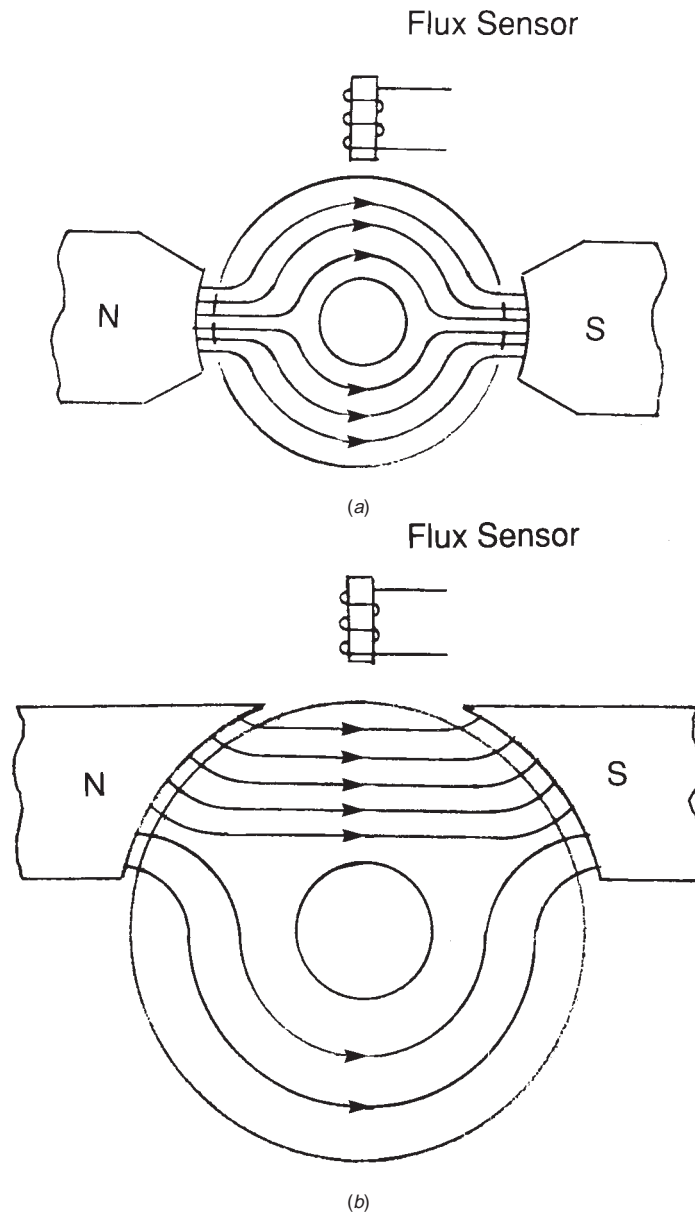
FIG. 1 Transverse Magnetization
