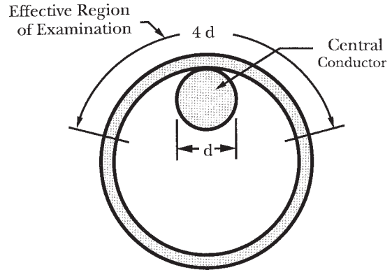
FIG. 16 Approximate Effective Region of Examination When Using an Offset Central Conductor (Threader Bar)
