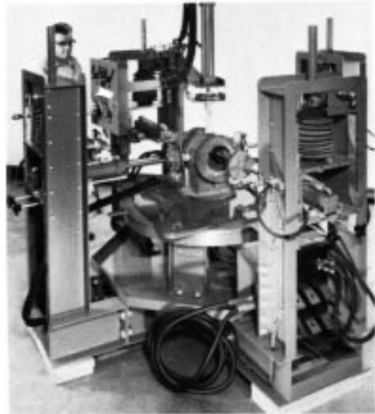
FIG. 7 Multidirectional—Overall Magnetization
