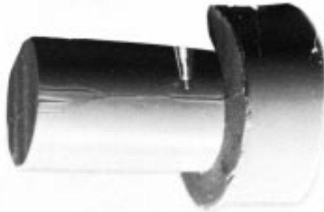
FIG. A1.13 Magnetic Rubber Indications of Surface Cracks in Aircraft Fastener Holes (Produced by Yoke Magnetization DC Continuous)
