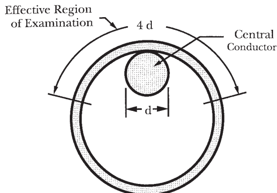
FIG. 17 16 Approximate Effective Region of Examination When Using an Offset Central Conductor (Threader Bar)
