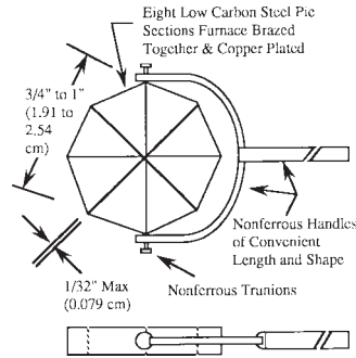
FIG. 15 Magnetic Field Indicator
