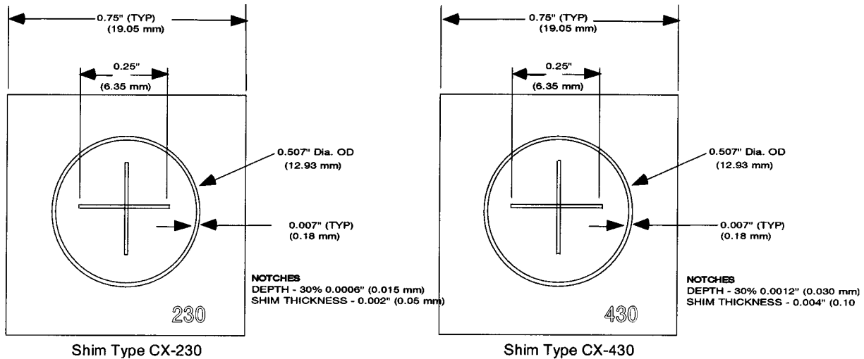
FIG. X1.2 Shim Types CX-230 and CX-430
