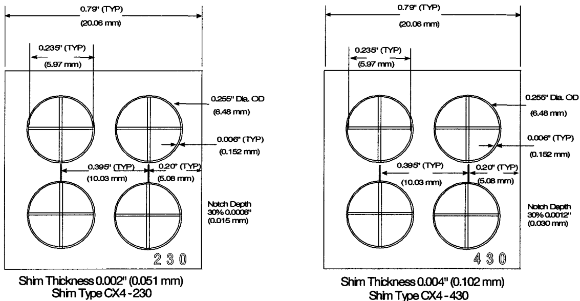
FIG. X1.3 Shim Thicknesses for Shim Types CX4-230 and CX4-430
