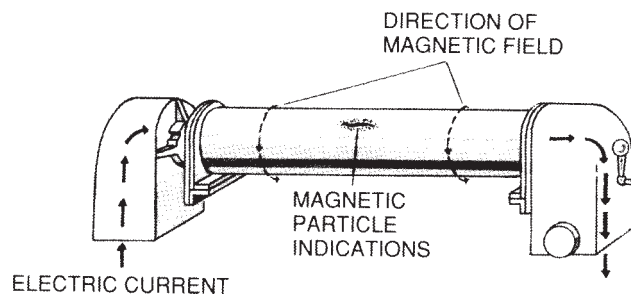
FIG. 10 Circular Magnetization
