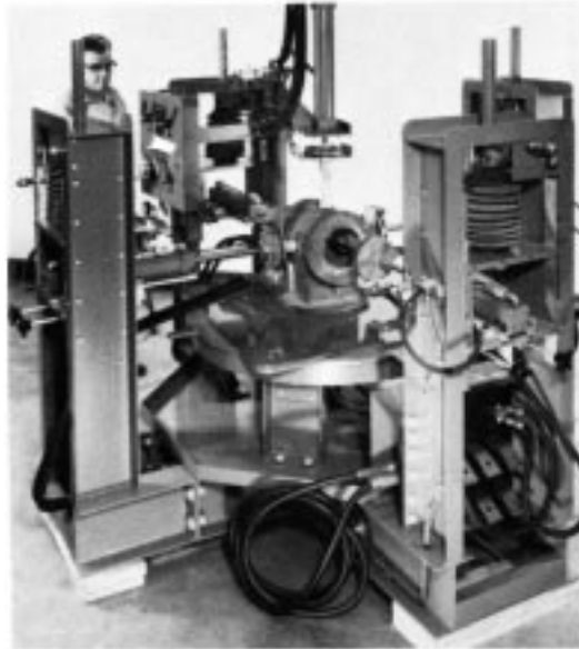
FIG. 7 Multidirectional–Overall Magnetization
