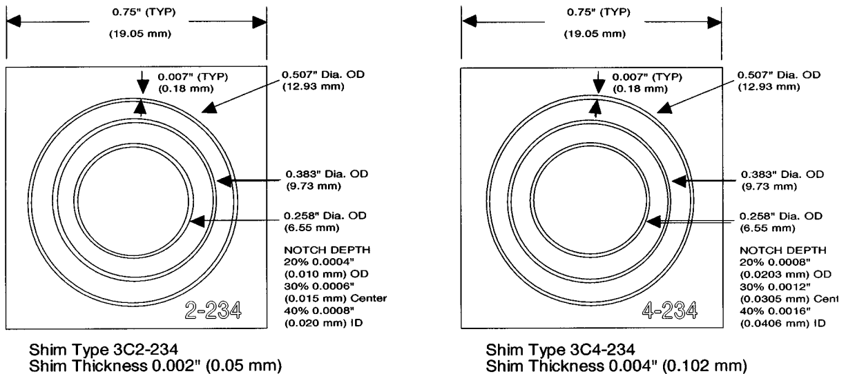
FIG. X1.1 Shim Thicknesses for Shim Types 3C2-234 and 3C4-234
