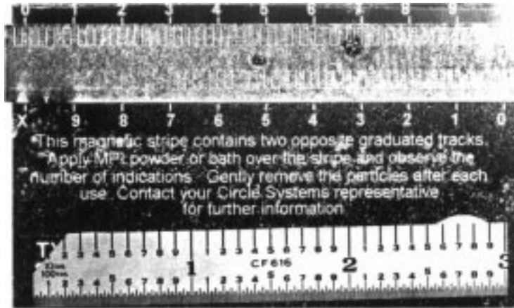
FIG. X2.1 Example of fluorescent particle indications of a decaying encoding pattern (top track) and a reverse-decaying pattern (bottom track) on the magnetic stripe of a magnetic stripe card.
