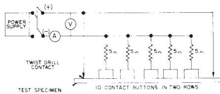
FIG. 2 Diagram of Connections for Contacts and Resistors
