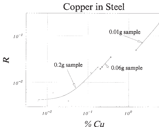
FIG. A3.2 Neocuproine Copper Method
