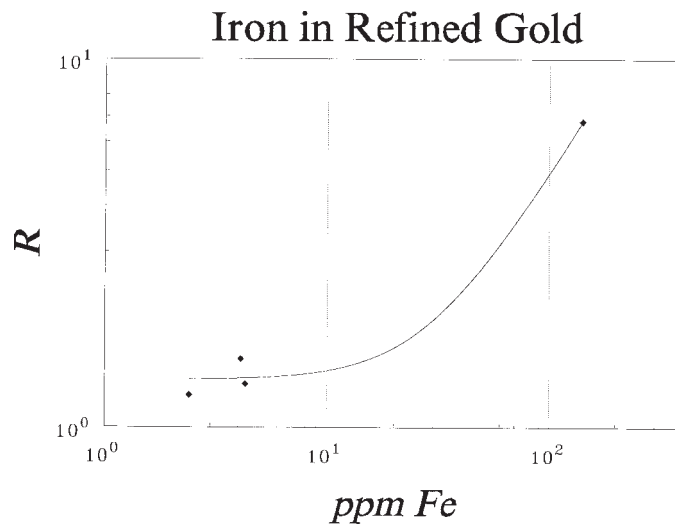
FIG. A2.2 R for Iron in Refined Gold
