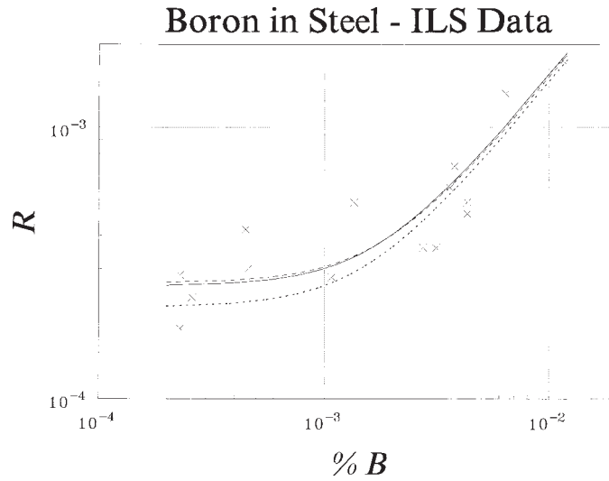
FIG. A2.1 Variation of Reproducibility Index with Analyte Concentration—General Model
