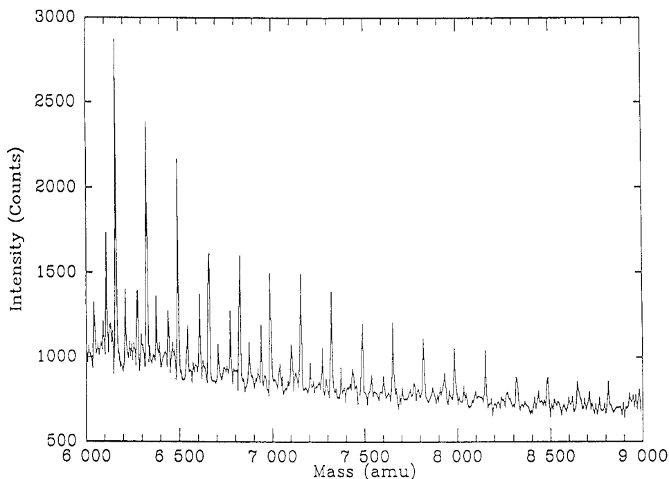
FIG. 1 Static SIMS Mass Spectrum of Perfluorinated Polyakylether
