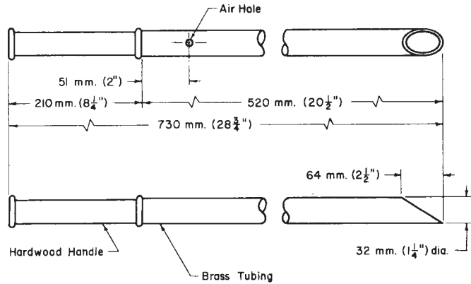
FIG. 2 Tube Sampler for Packaged Cement
