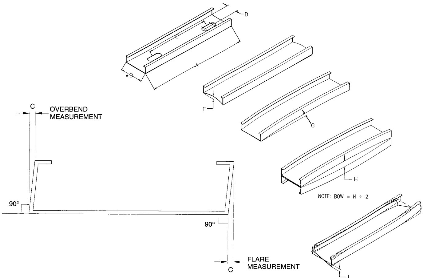
FIG. 1 Manufacturing Tolerances
