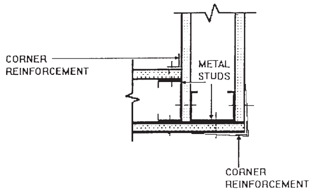
FIG. 2 Partition Corner Detail
