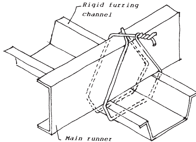
FIG. 10 Saddle Tie
