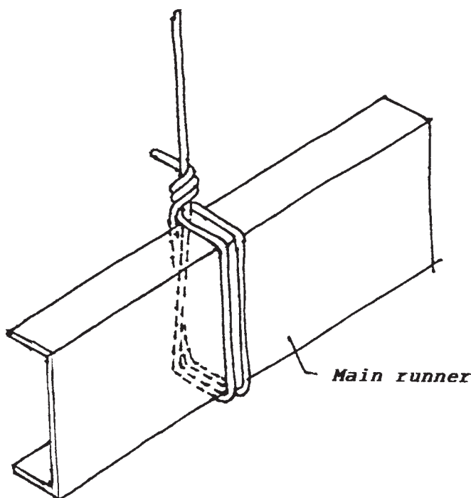
FIG. 4 Saddle Tie
