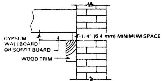
FIG. 9 Masonry Wall
