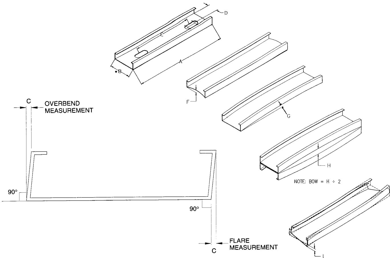
FIG. 2 Manufacturing Tolerances
