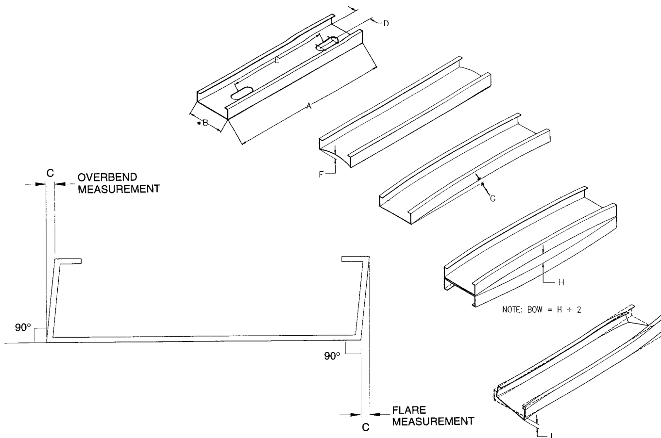
FIG. 2 Manufacturing Tolerances
