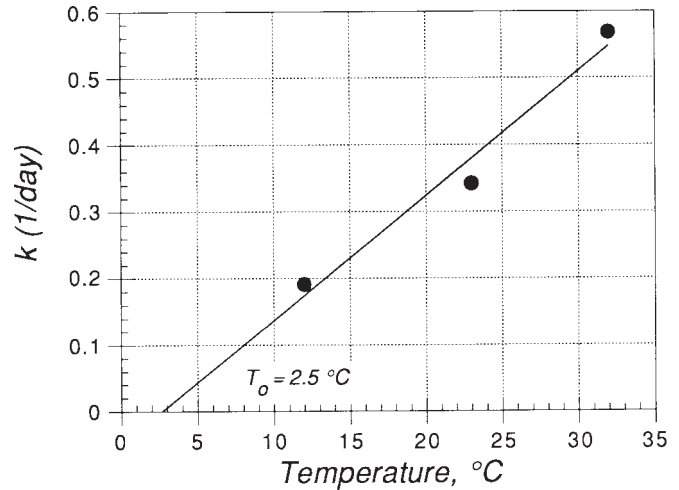
FIG. A1.2 Example of Plot of K -Values Versus Curing Temperature for Determining the Datum Temperature
