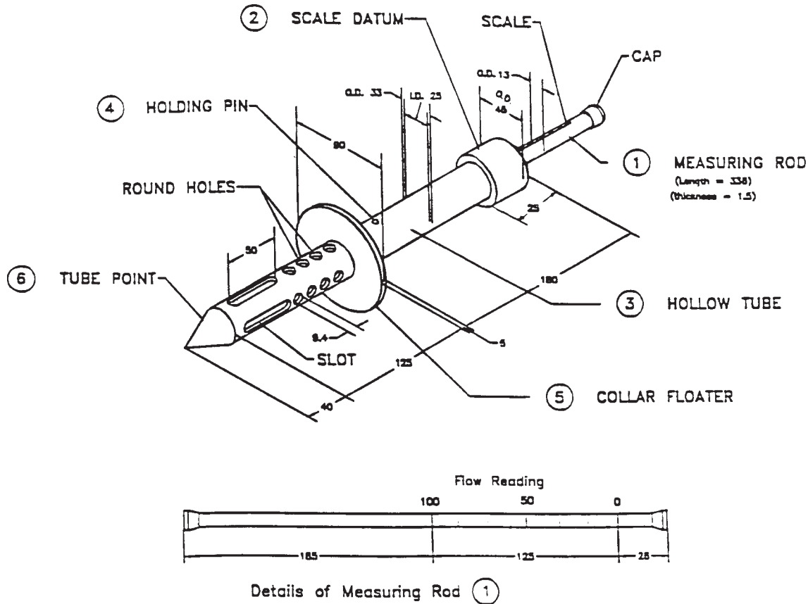
All dimensions in millimetres (1 in. = 25.4 mm) FIG. 1 Apparatus for Flow Test
