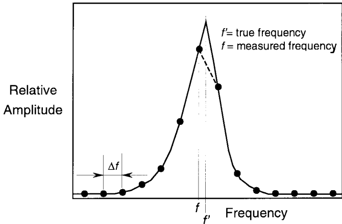
FIG. X1.3 Schematic of Amplitude Spectrum Resulting from an Impact-Echo (Procedure B) Test on a Solid Plate
