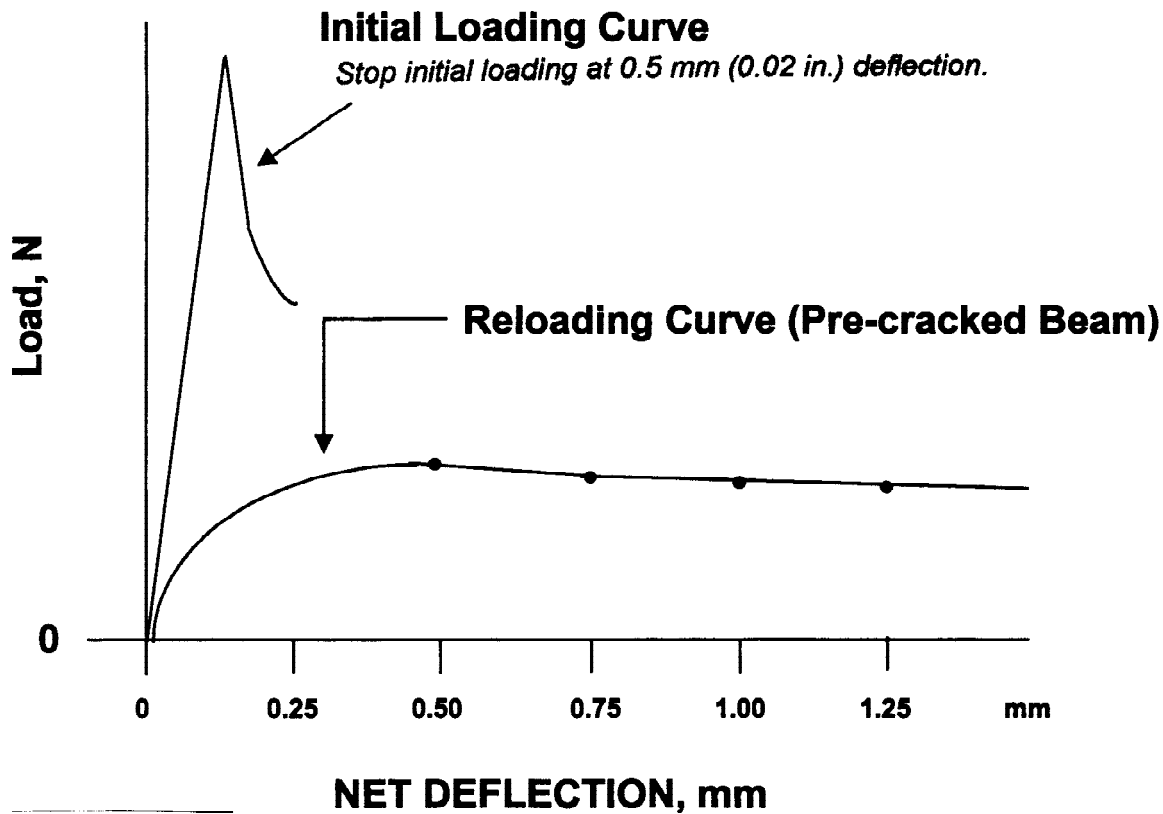
FIG. 2 3 Load-Deflection Curves
