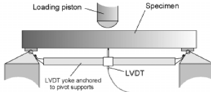
FIG. A1.1 Suggested Method of Deflection Measurement to Exclude Load-Train Deformations and Crushing of Concrete at the Point of Loading Using a Linear Variable Deflection Transducer (LVDT)
