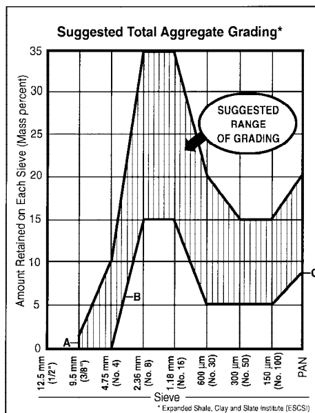
FIG. X1.1 Suggested Total Aggregate Grading
