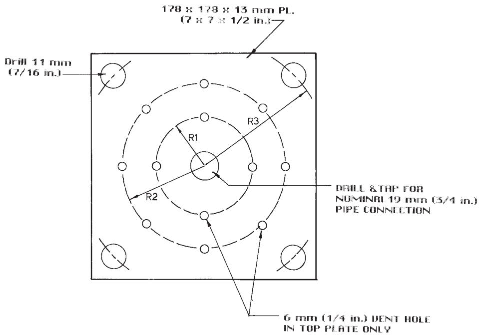
FIG. 1 Cylinder Mold Assembly Cross Section
