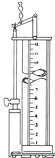
FIG. 2 Thief Sampler
