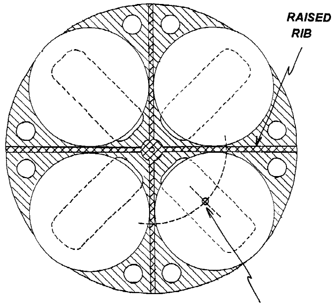
APPROXIMATELY TO SCALE FIG. X1.2 Recommended TFOT Shelf With Four Pans
