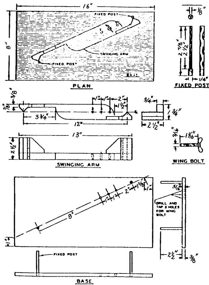
FIG. 1 Proportional Caliper
