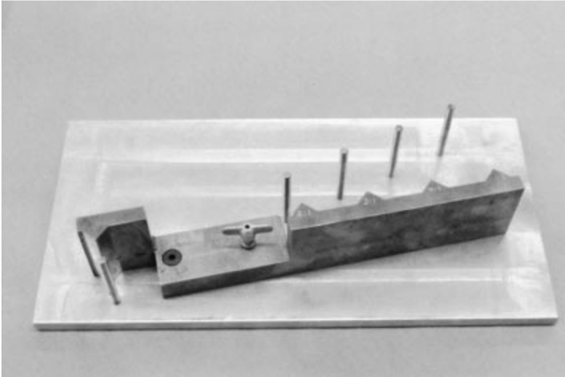
FIG. 3 Proportional Caliper
