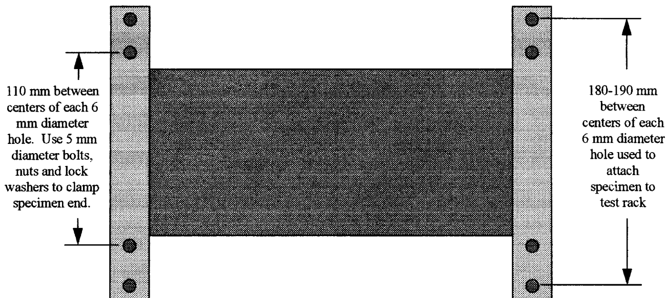
FIG. 1 Diagram Showing Clamping Bars Used for Attaching Type VI Shheeting Specimens to Test Rack for Outdoor Exposure
