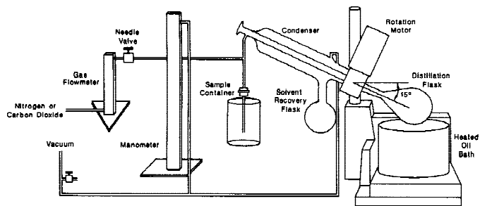
FIG. 1 Rotary Evaporator and Recovery System
