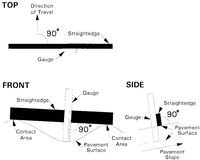
NOTE 1— Fig. 1 represents only one type of rut configuration. FIG. 1 Rut Configuration
