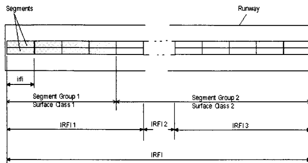
FIG. 1 Illustration of a Segmented Runway
