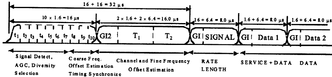
FIG. 8 OFDM Training Structure
