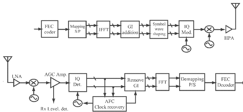
FIG. 10 Transmitter and Receiver Block Diagram for the OFDM PHY
